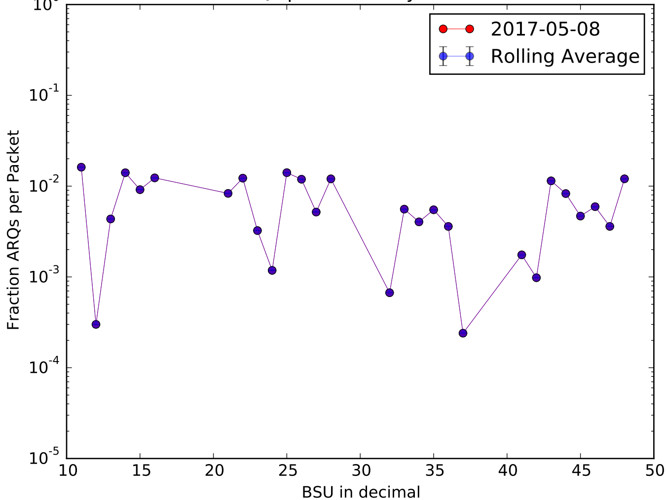
Fraction ARQs per Packet by BSU 2017-05-08
