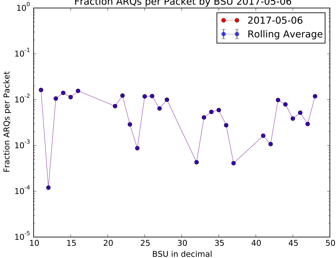
Fraction ARQs per Packet by BSU 2017-05-06
