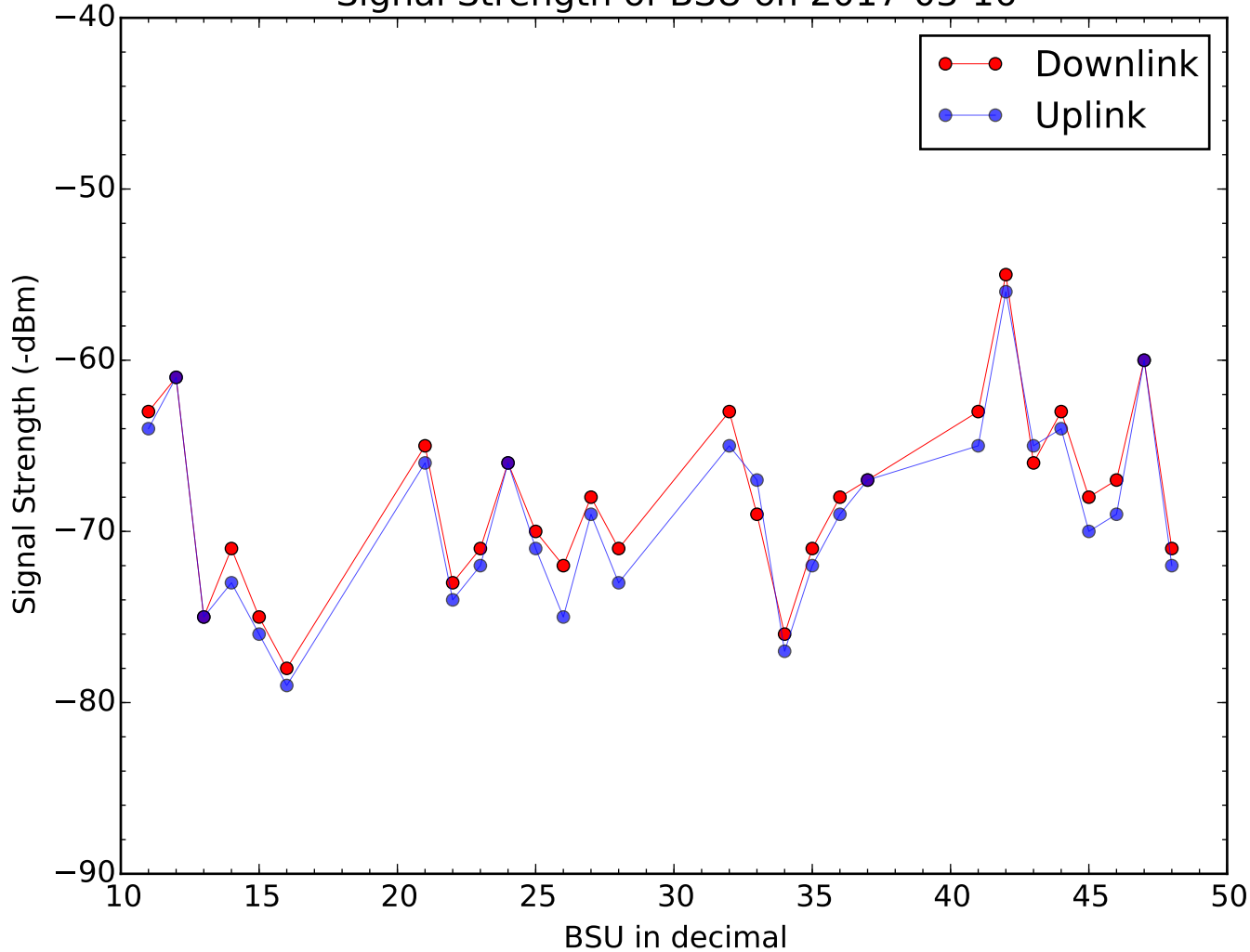
Signal Strength of BSU on 2017-03-16
