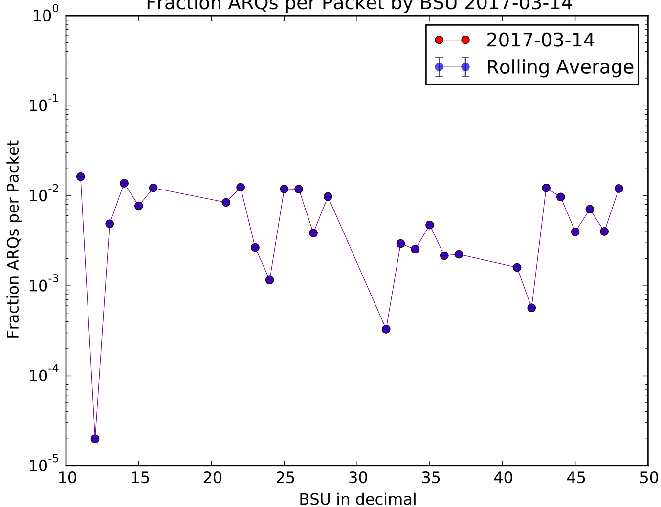
Fraction ARQs per Packet by BSU 2017-03-14
