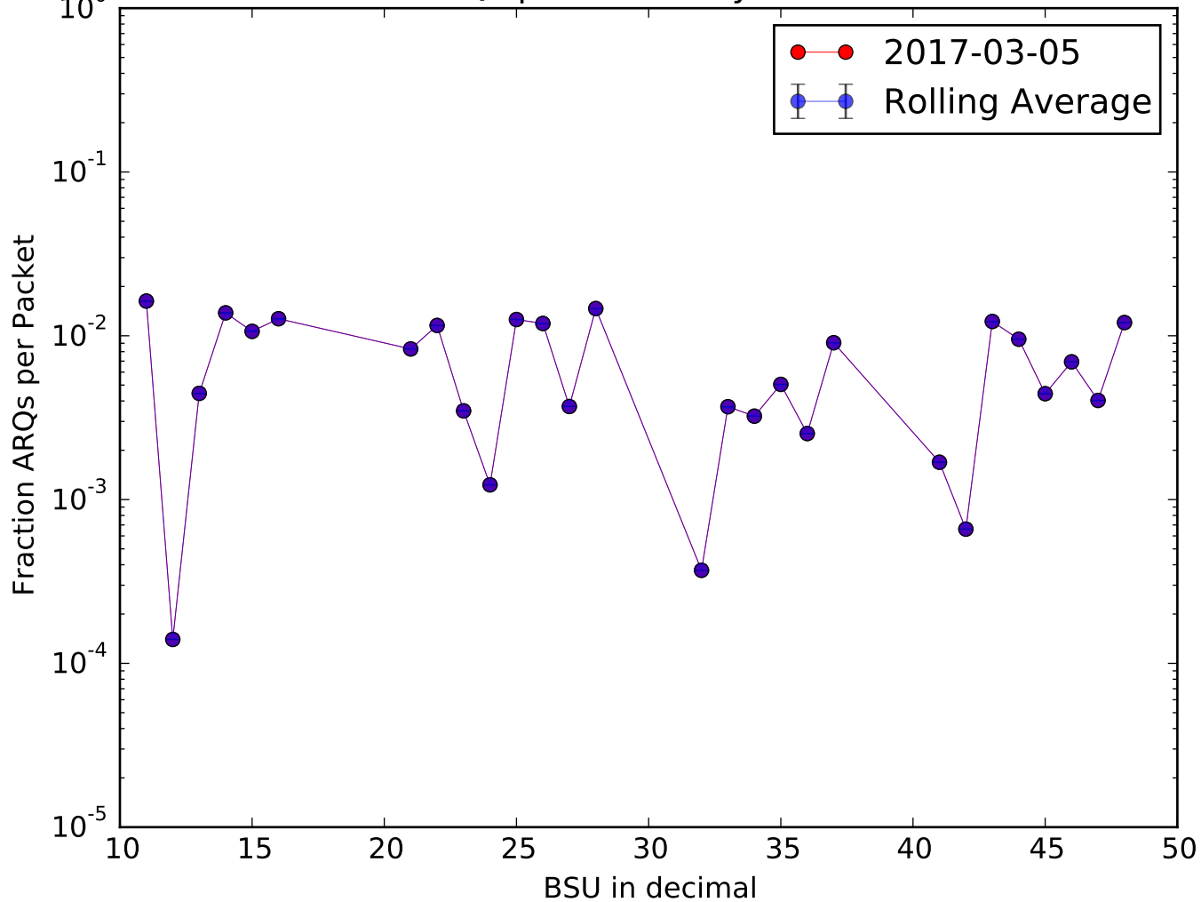
Fraction ARQs per Packet by BSU 2017-03-05
