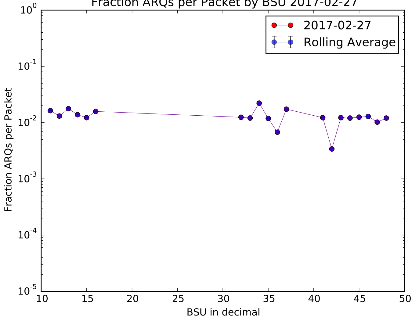
Fraction ARQs per Packet by BSU 2017-02-27
