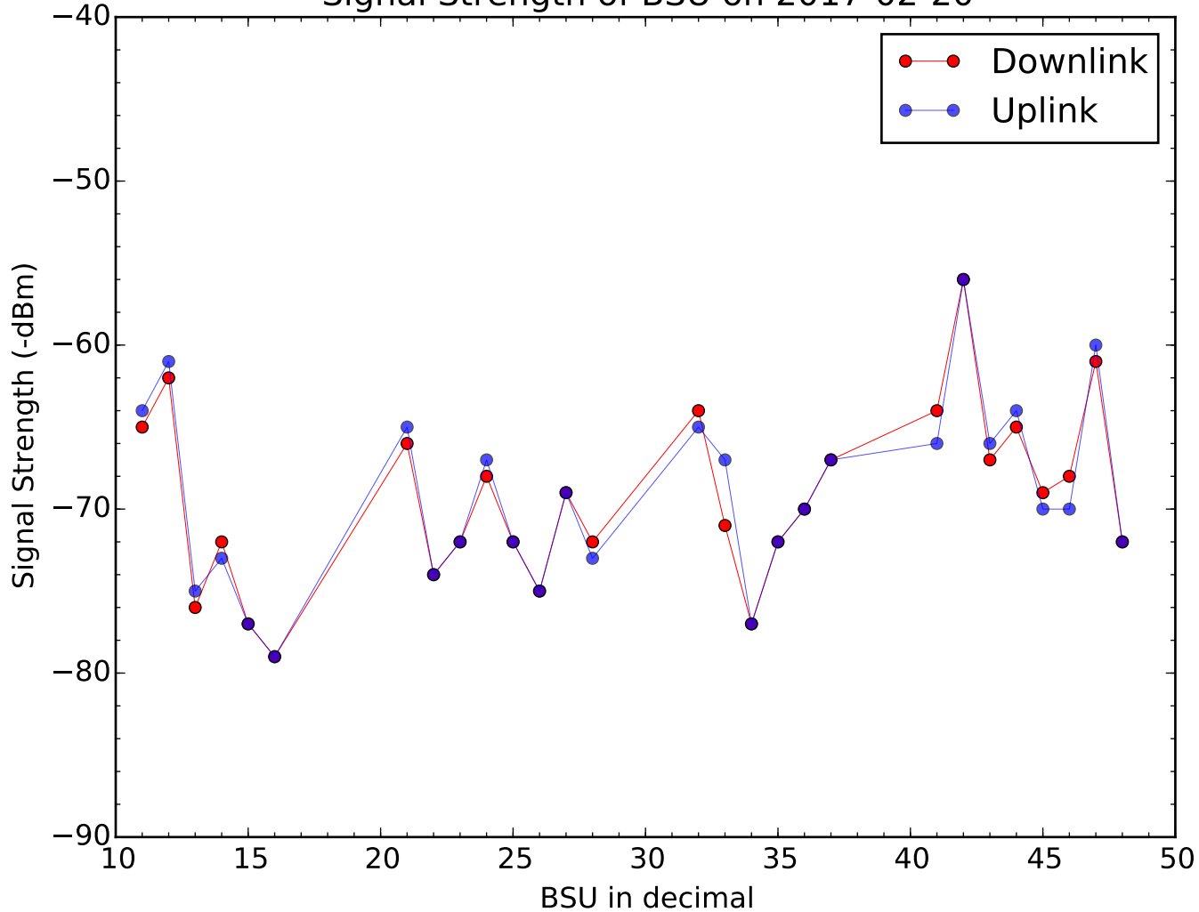
Signal Strength of BSU on 2017-02-20
