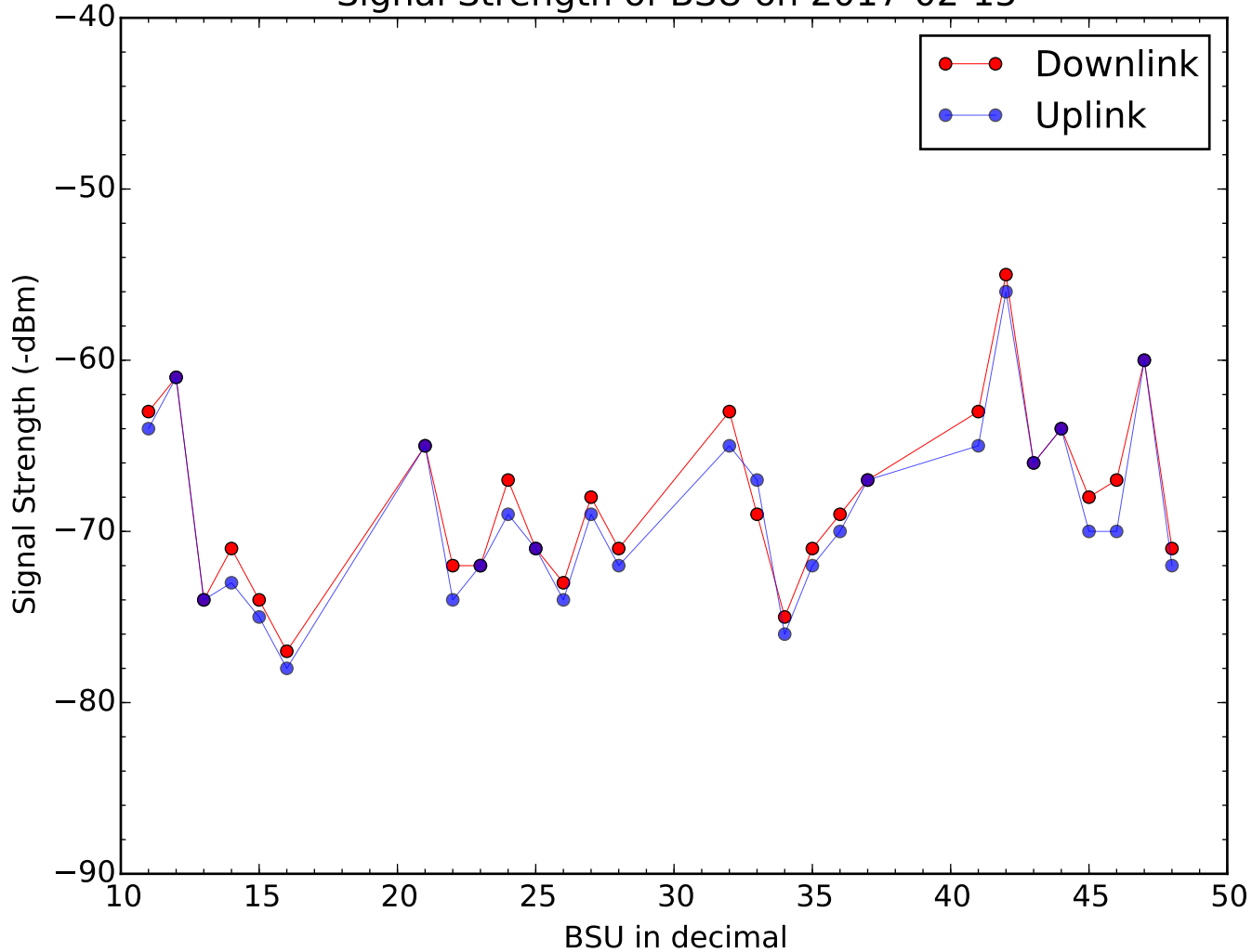
Signal Strength of BSU on 2017-02-15
