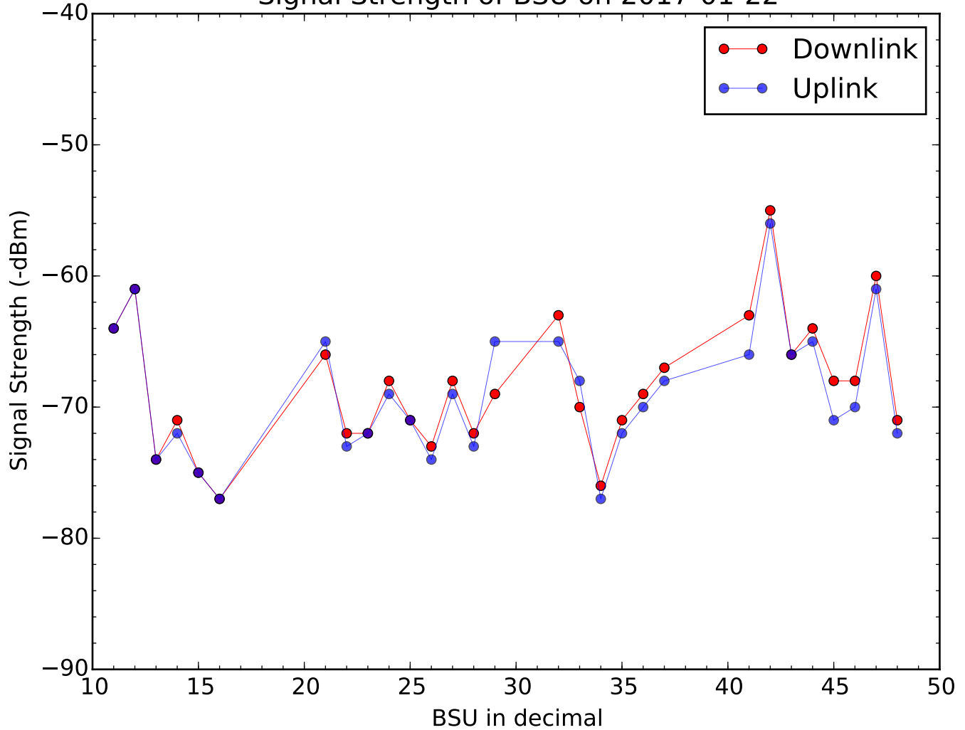
Signal Strength of BSU on 2017-01-22
