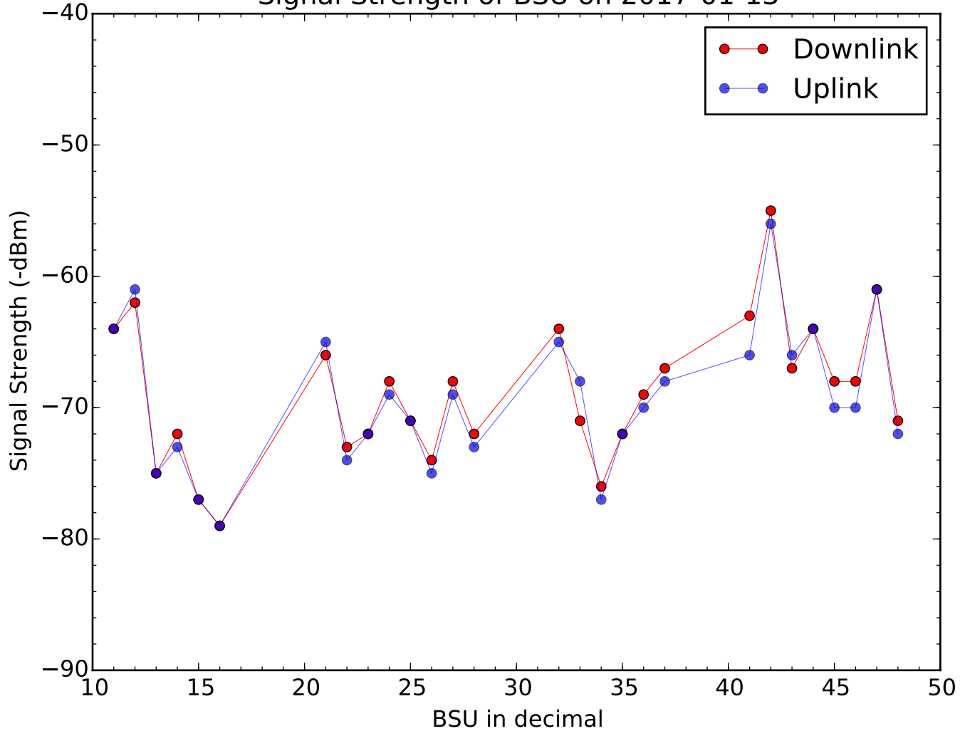
Signal Strength of BSU on 2017-01-13
