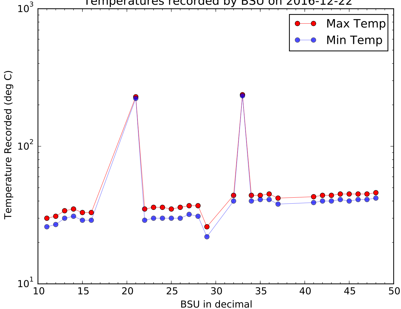
Temperatures recorded by BSU on 2016-12-22
