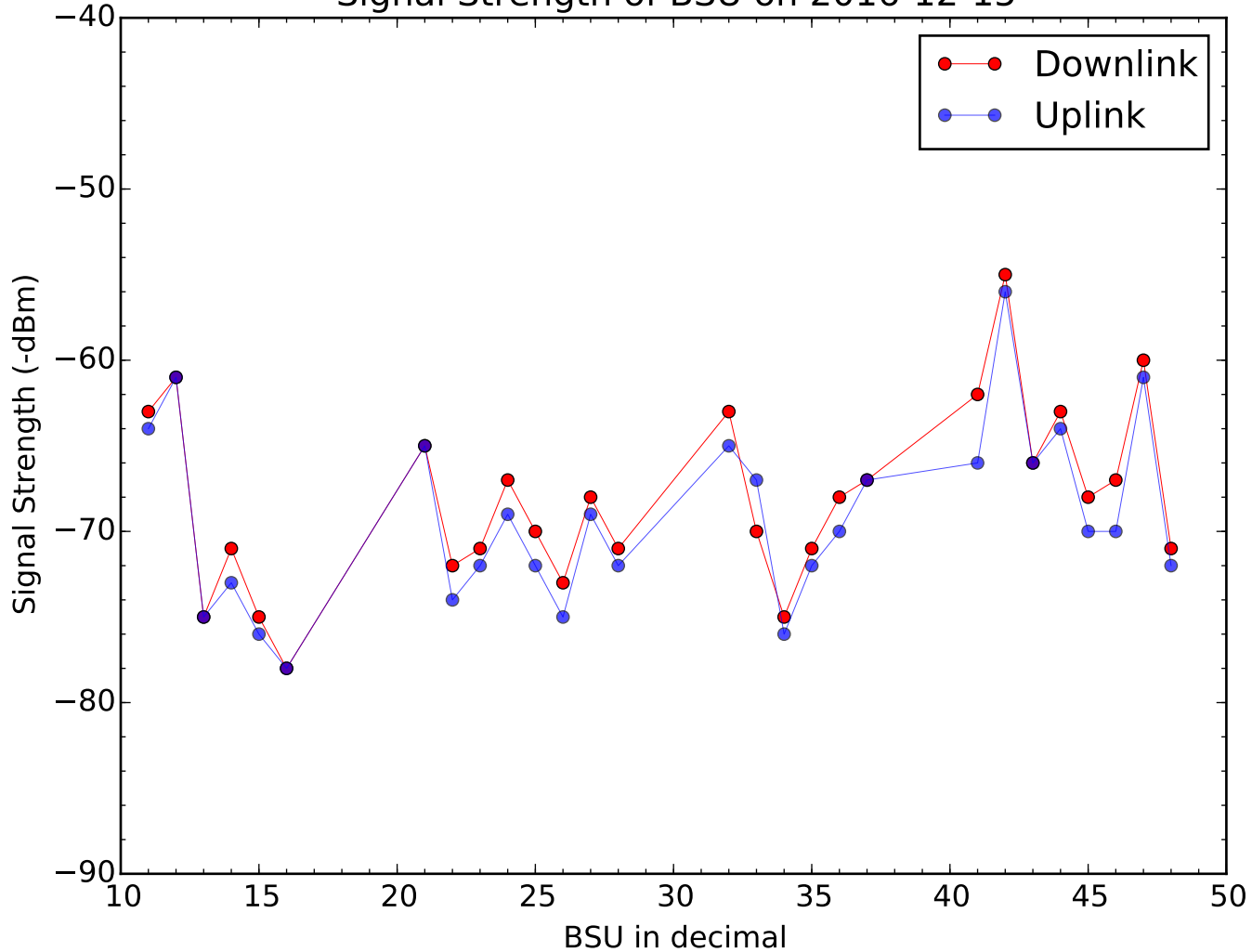
Signal Strength of BSU on 2016-12-15
