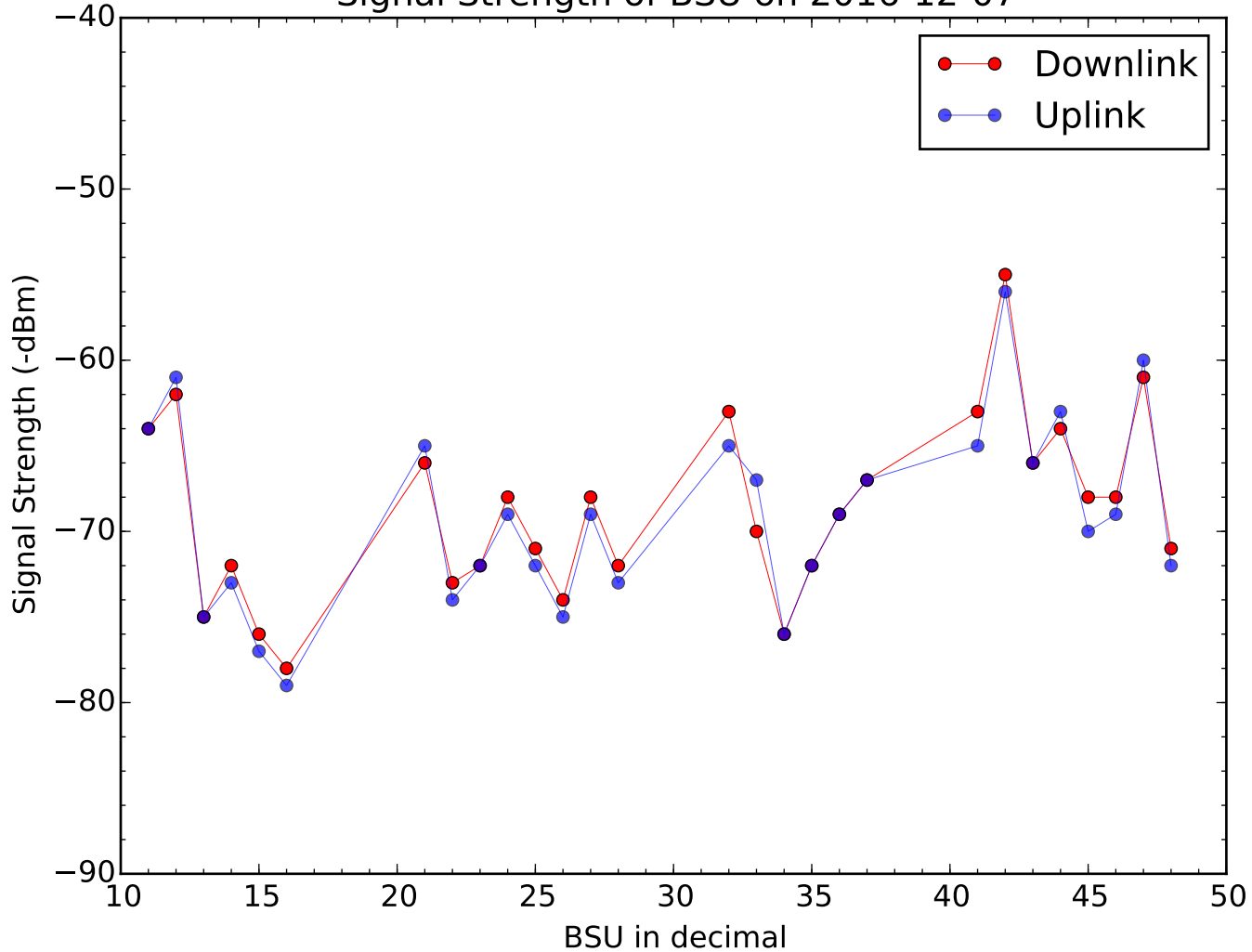
Signal Strength of BSU on 2016-12-07
