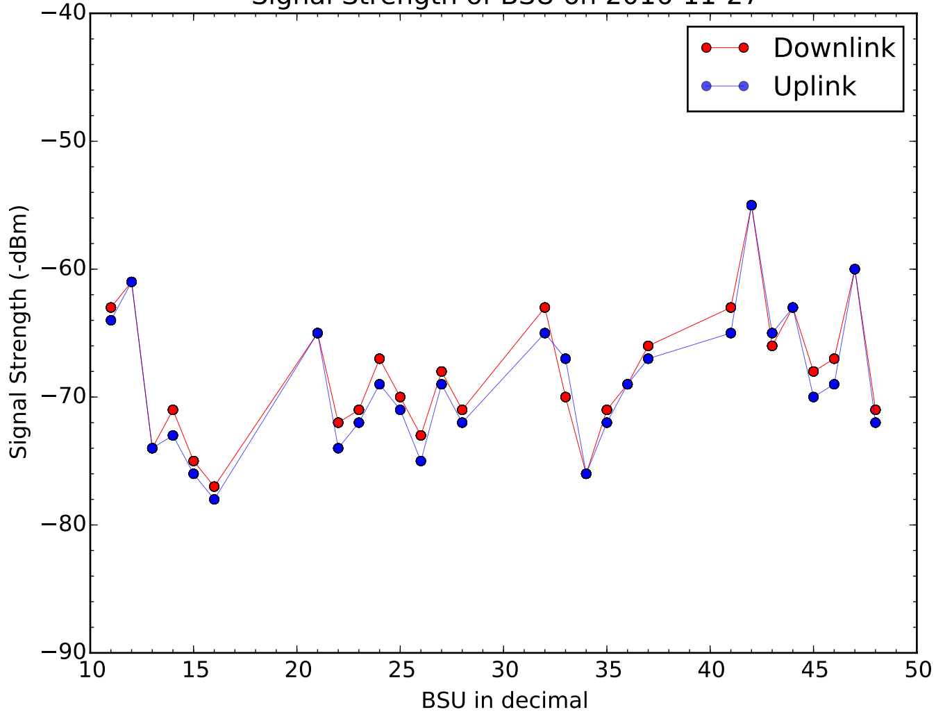
Signal Strength of BSU on 2016-11-27
