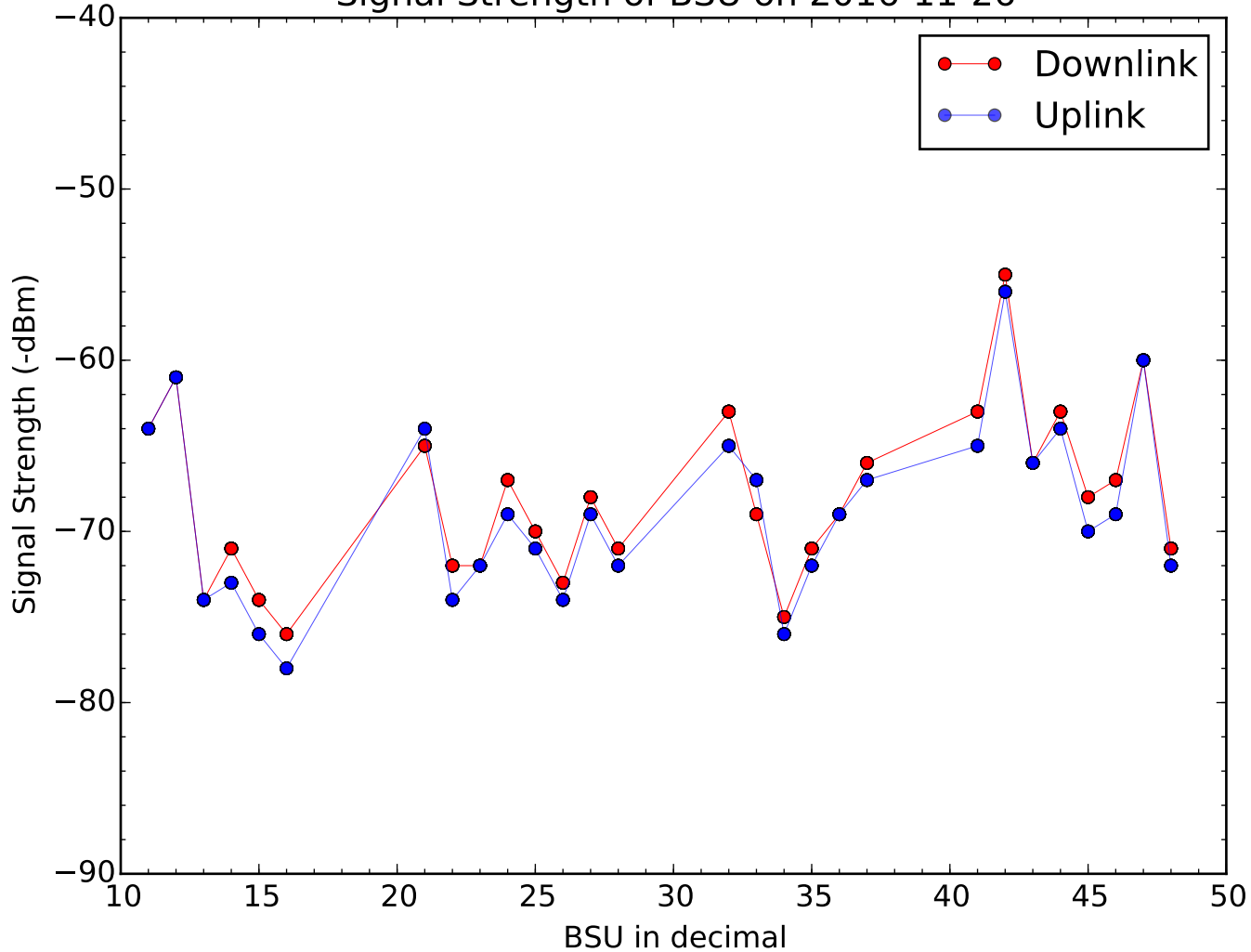
Signal Strength of BSU on 2016-11-26
