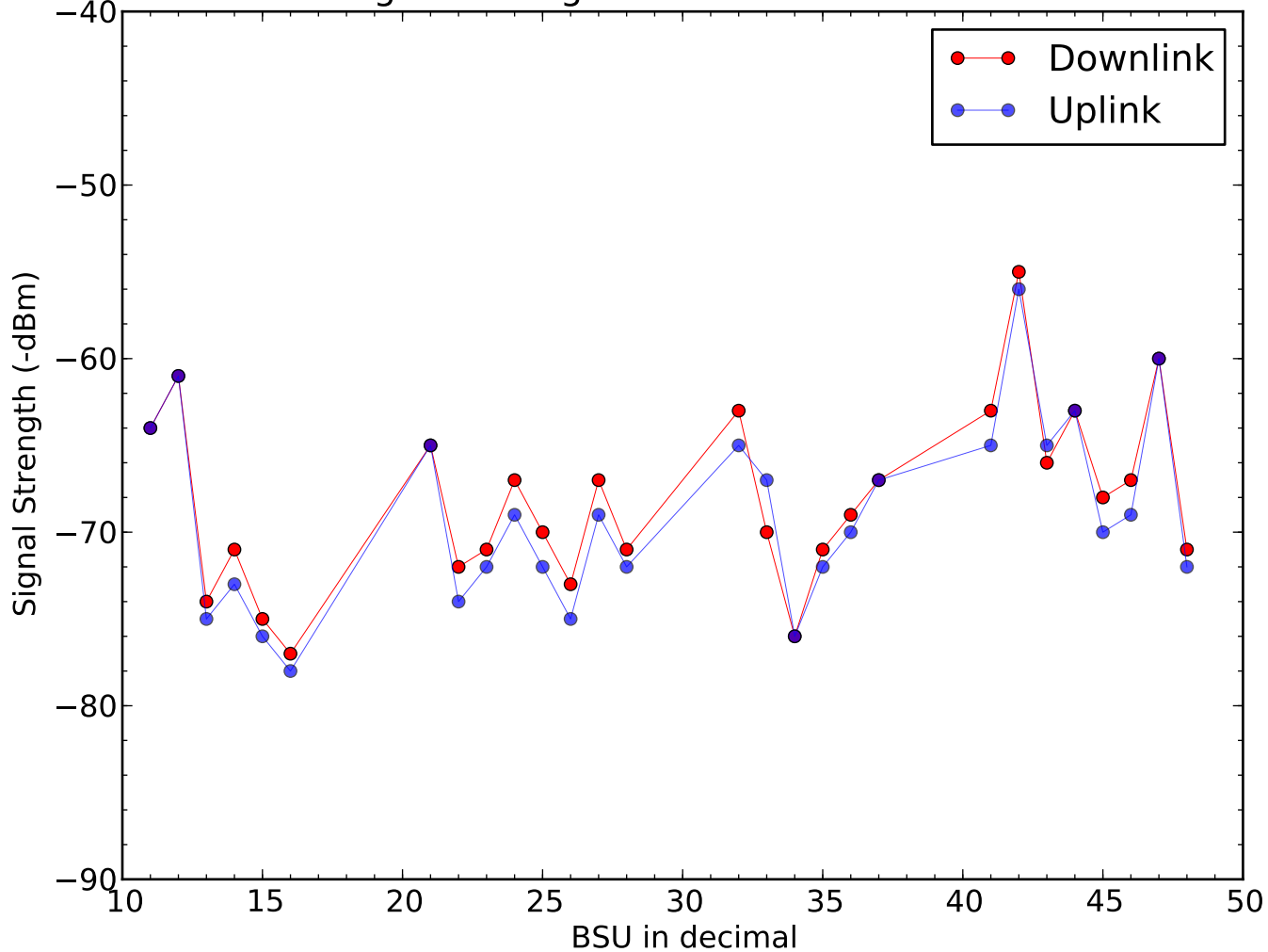
Signal Strength of BSU on 2016-11-16
