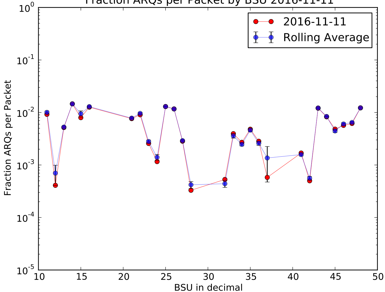
Fraction ARQs per Packet by BSU 2016-11-11
