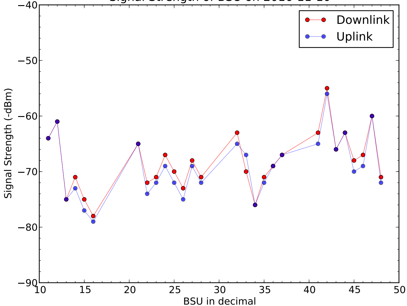
Signal Strength of BSU on 2016-11-10
