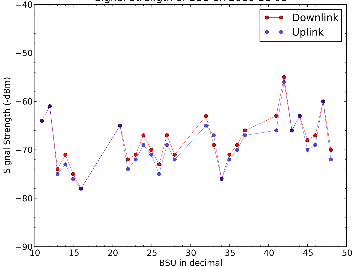
Signal Strength of BSU on 2016-11-08
