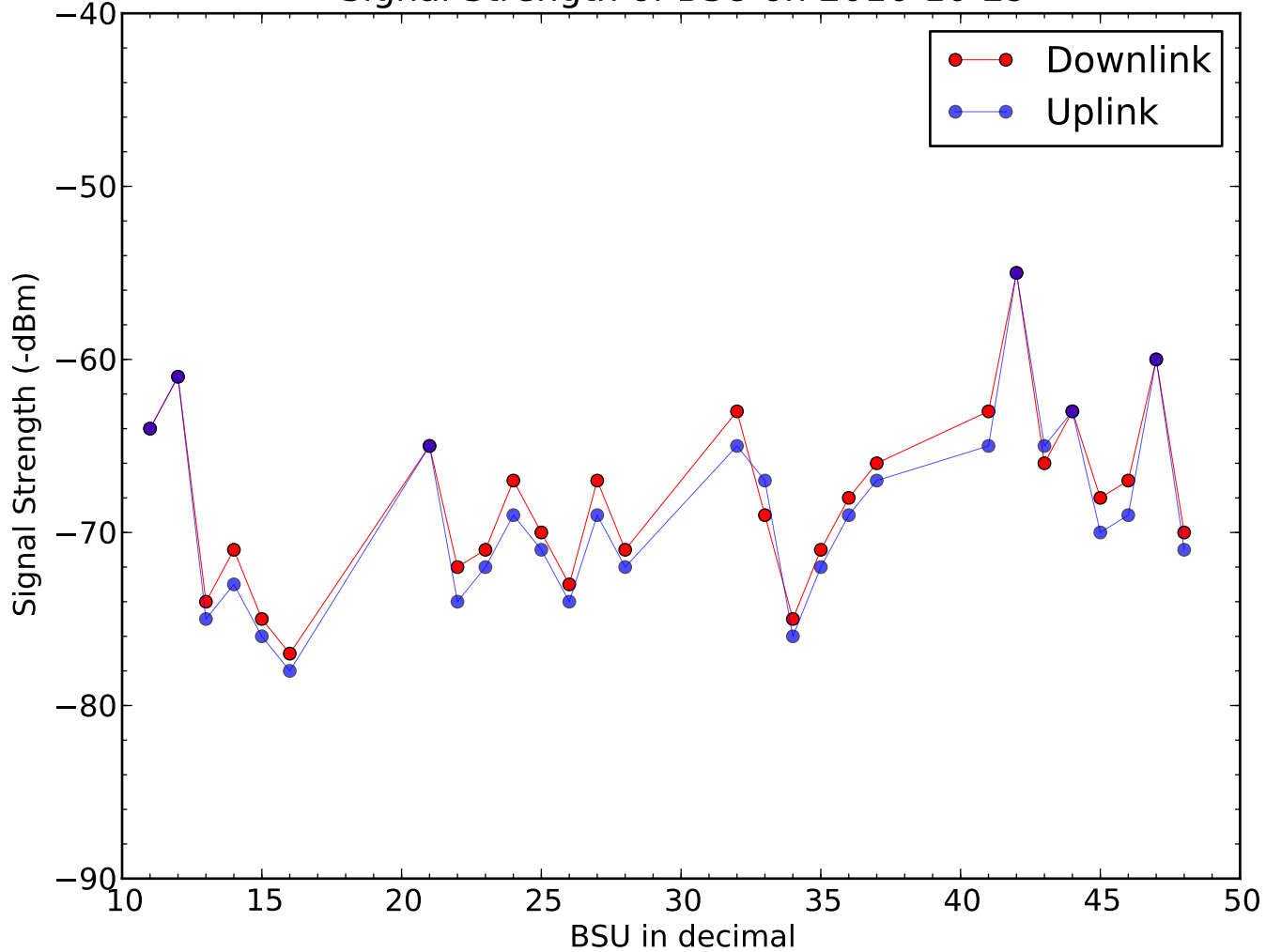
Signal Strength of BSU on 2016-10-29
