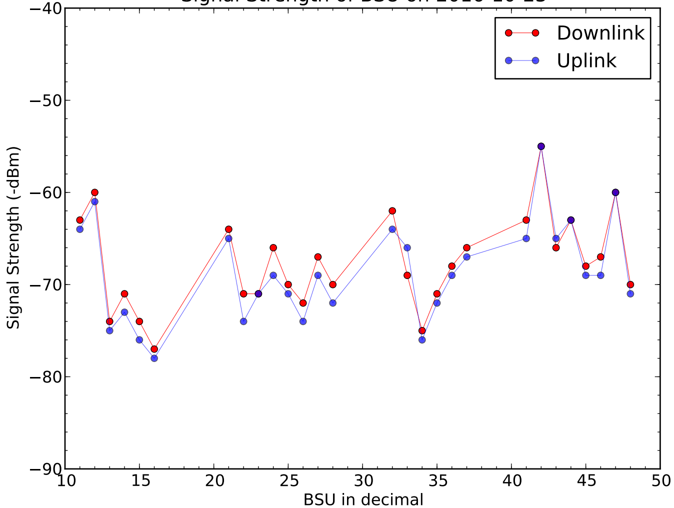
Signal Strength of BSU on 2016-10-23
