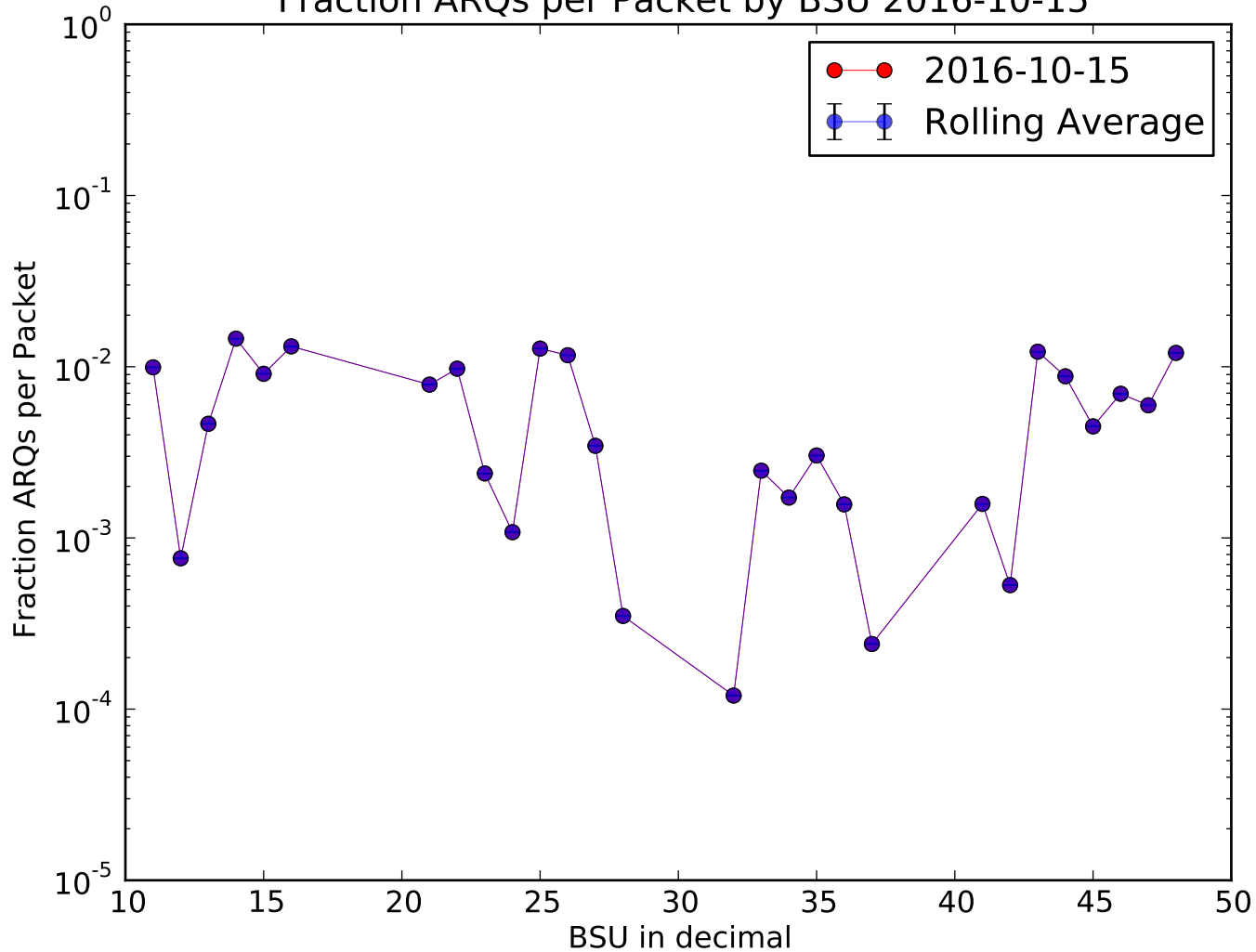
Fraction ARQs per Packet by BSU 2016-10-15
