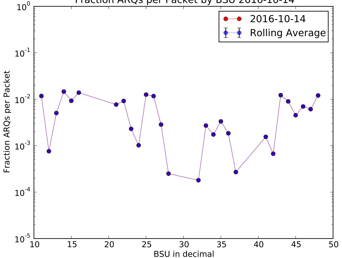
Fraction ARQs per Packet by BSU 2016-10-14
