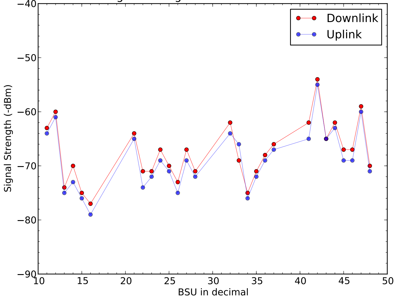
Signal Strength of BSU on 2016-10-09
