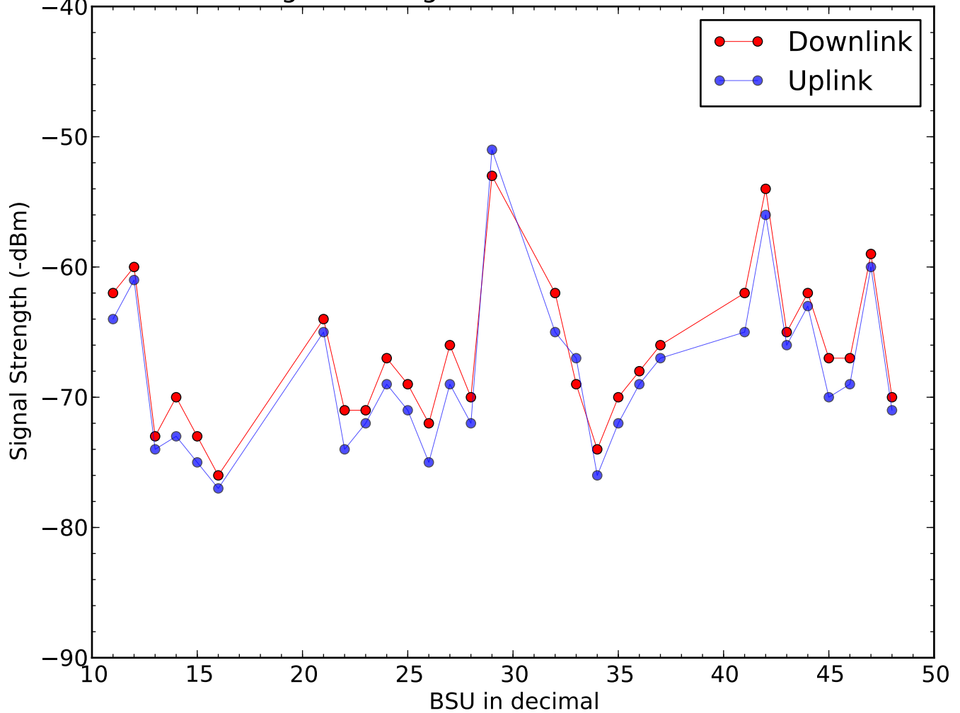
Signal Strength of BSU on 2016-10-07
