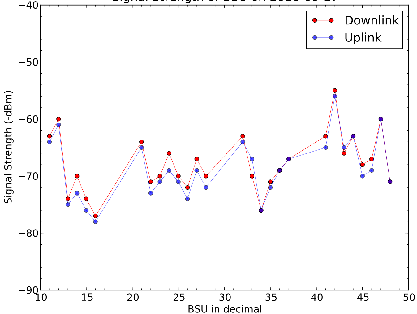
Signal Strength of BSU on 2016-09-27
