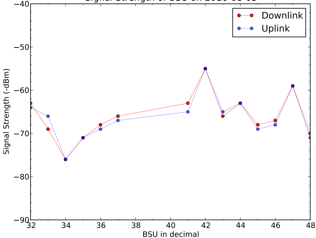
Signal Strength of BSU on 2016-08-03
