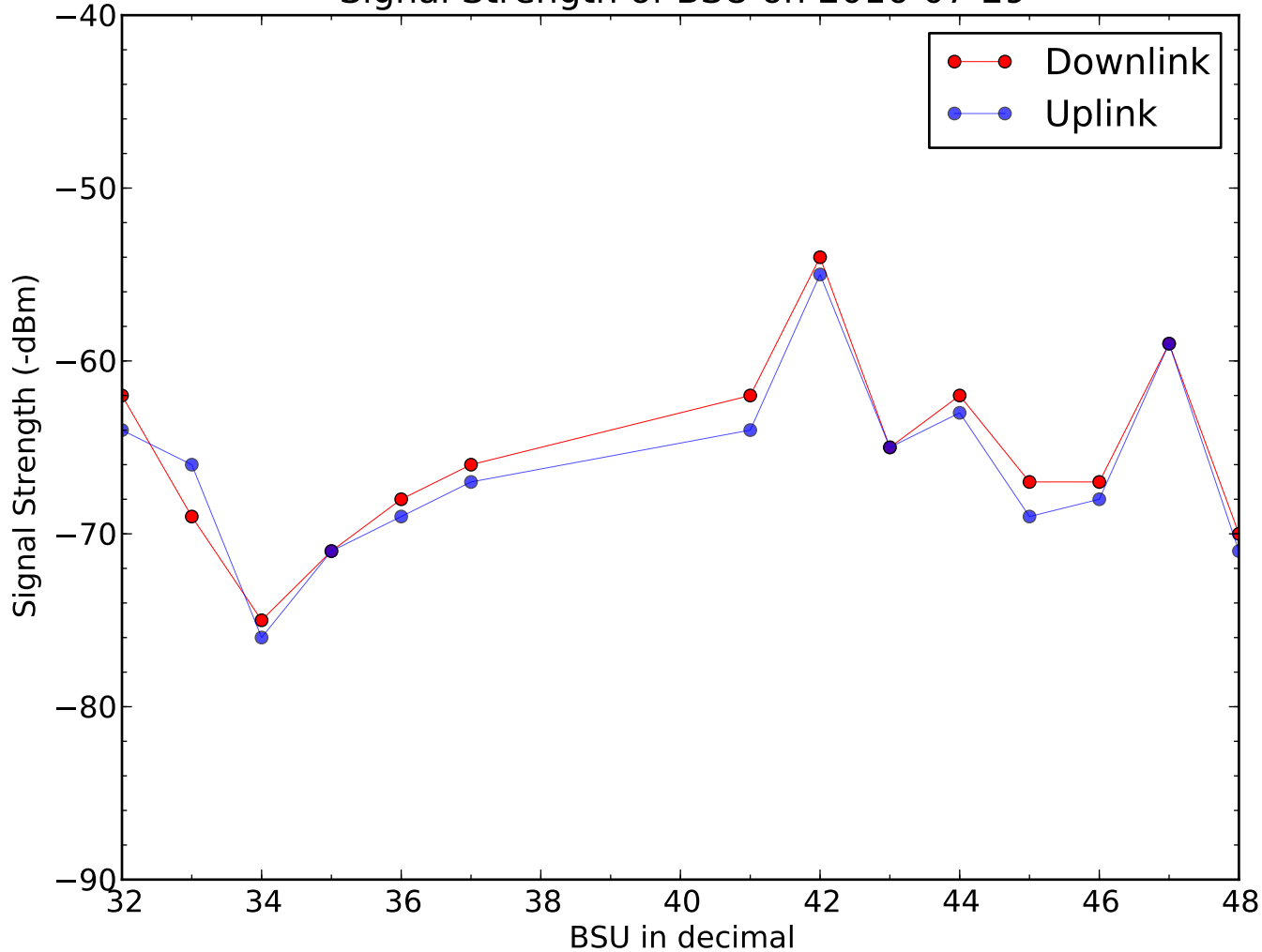
Signal Strength of BSU on 2016-07-29
