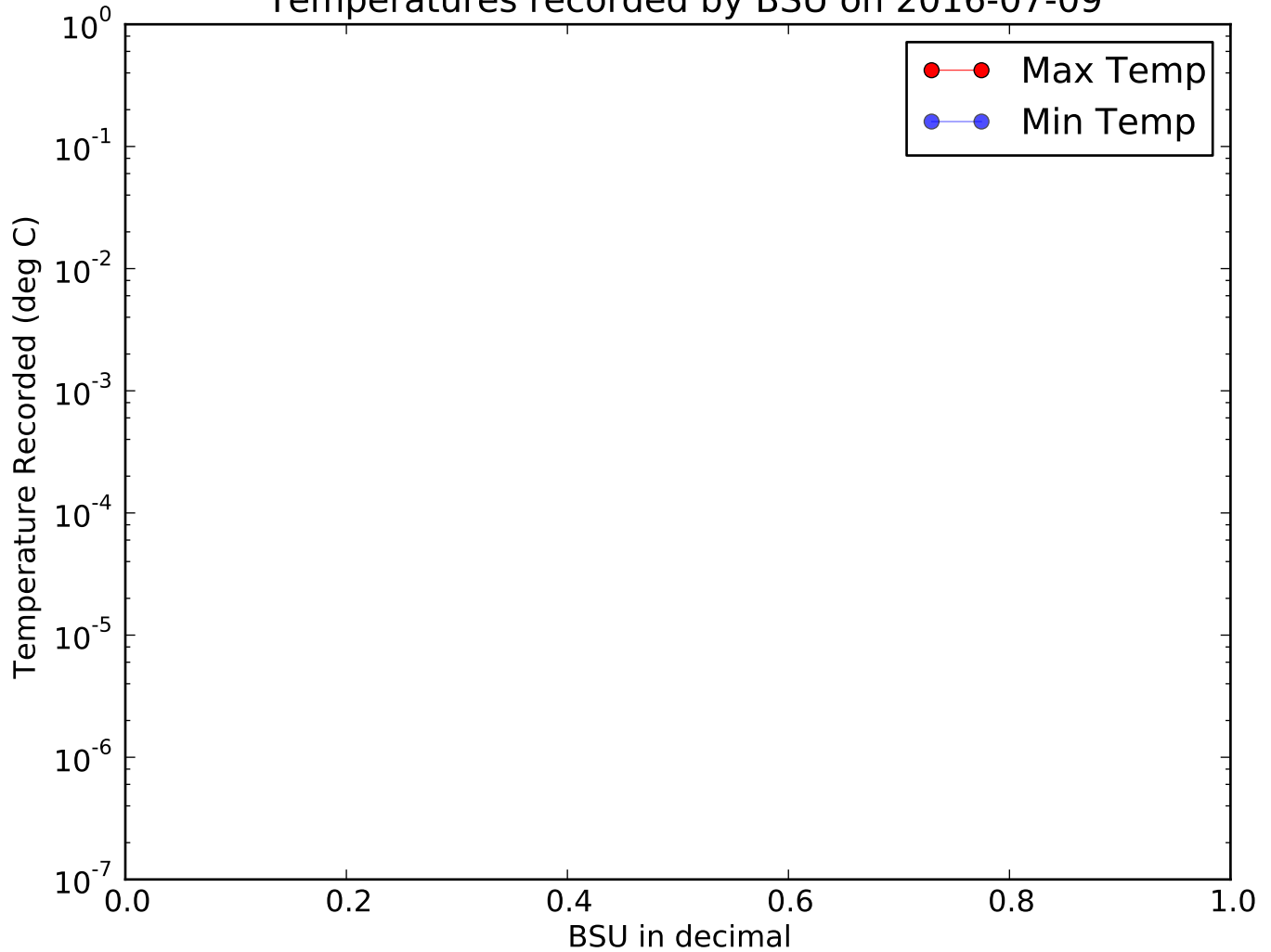
Temperatures recorded by BSU on 2016-07-09
