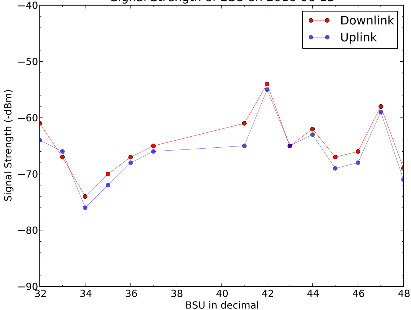
Signal Strength of BSU on 2016-06-13
