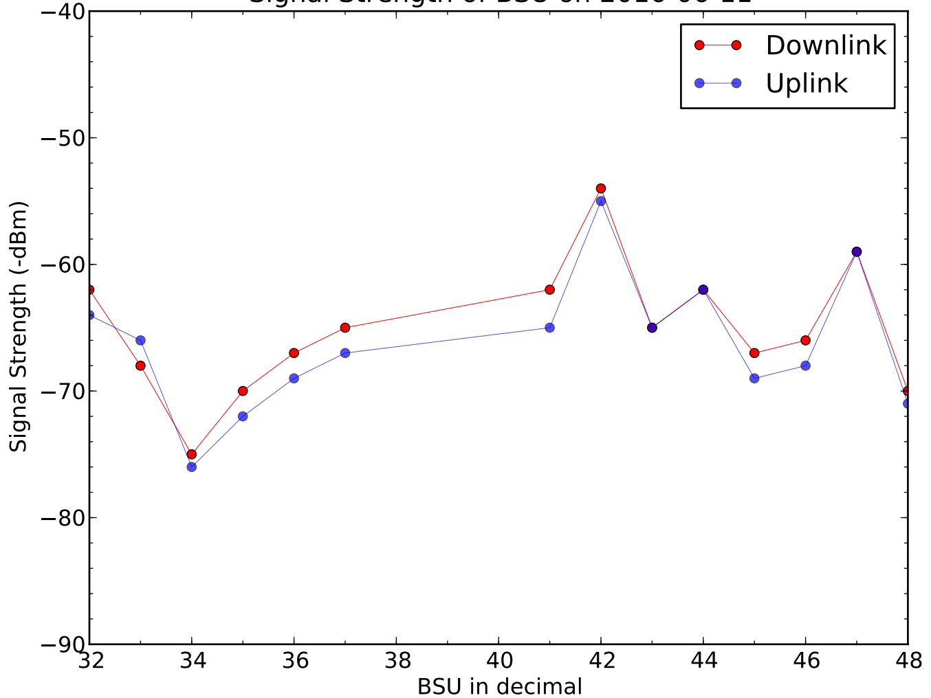
Signal Strength of BSU on 2016-06-11
