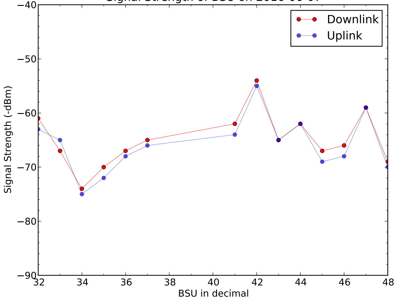
Signal Strength of BSU on 2016-06-07
