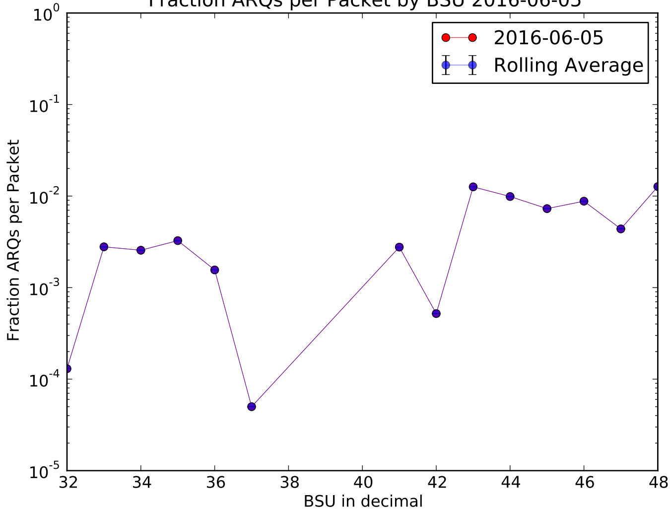
Fraction ARQs per Packet by BSU 2016-06-05
