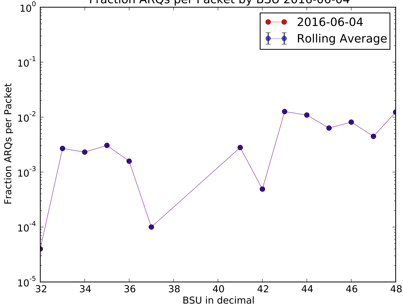
Fraction ARQs per Packet by BSU 2016-06-04
