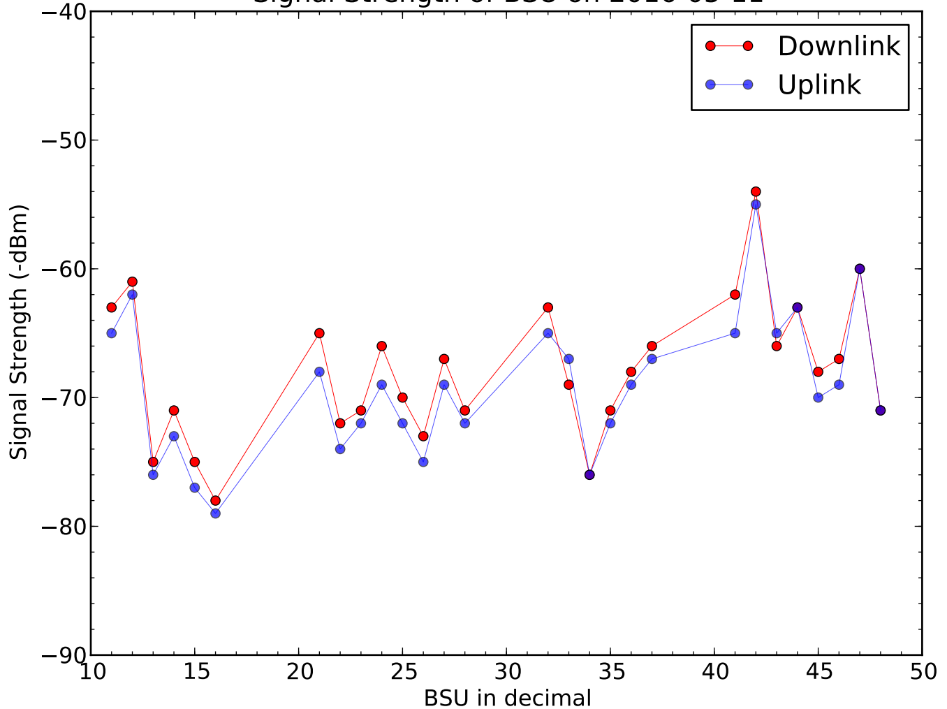
Signal Strength of BSU on 2016-05-11
