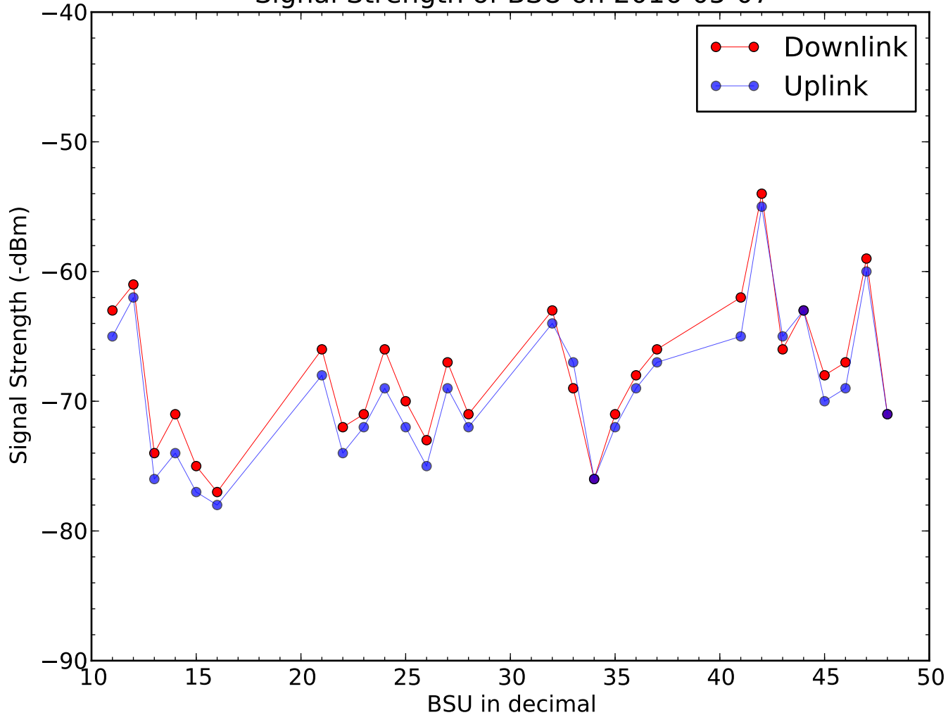
Signal Strength of BSU on 2016-05-07
