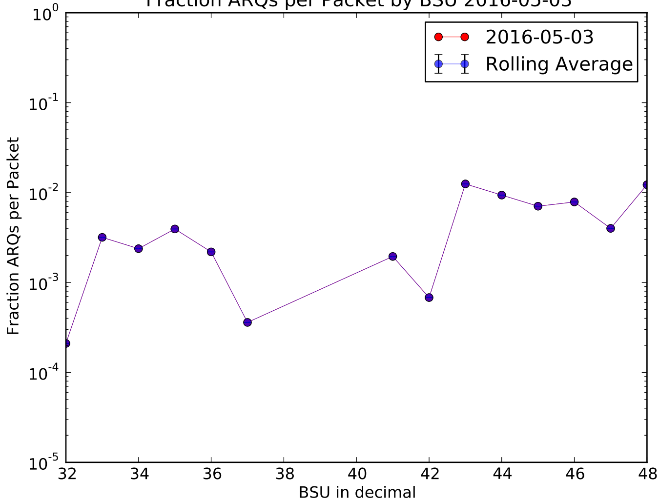
Fraction ARQs per Packet by BSU 2016-05-03
