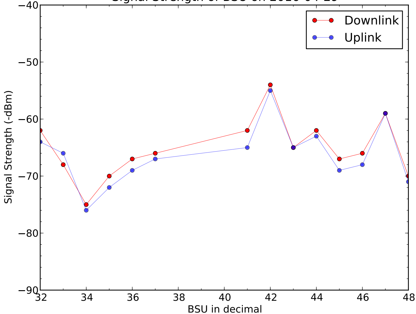
Signal Strength of BSU on 2016-04-29
