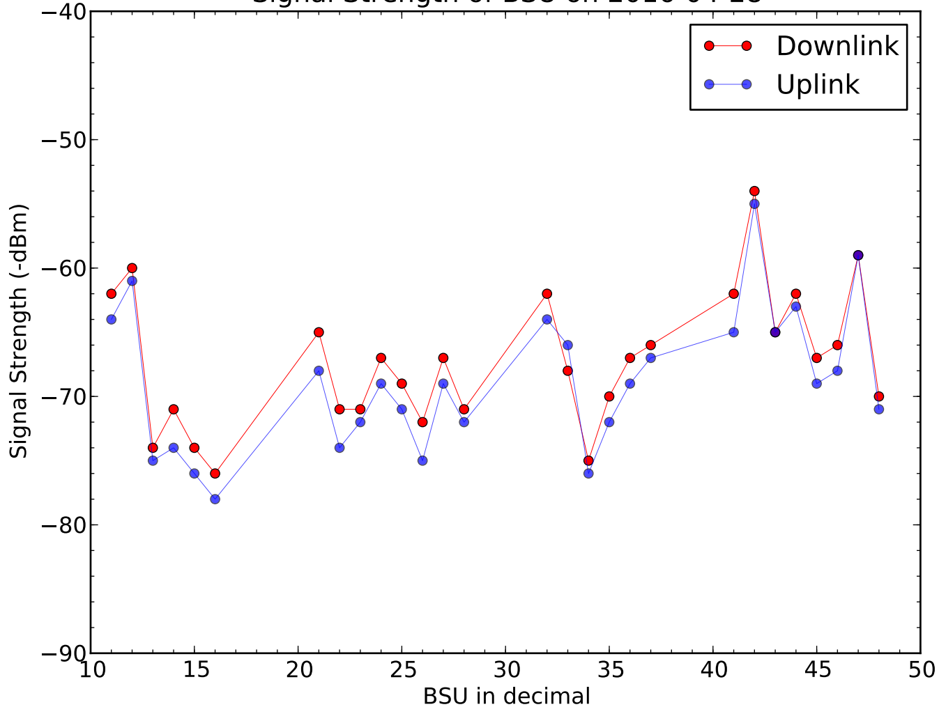
Signal Strength of BSU on 2016-04-28
