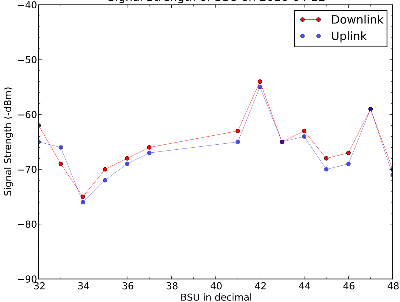
Signal Strength of BSU on 2016-04-22
