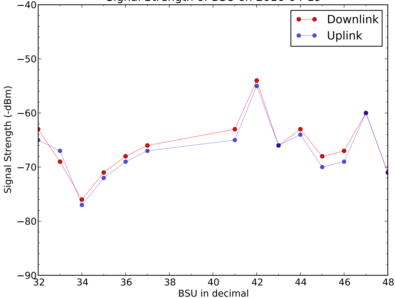
Signal Strength of BSU on 2016-04-19
