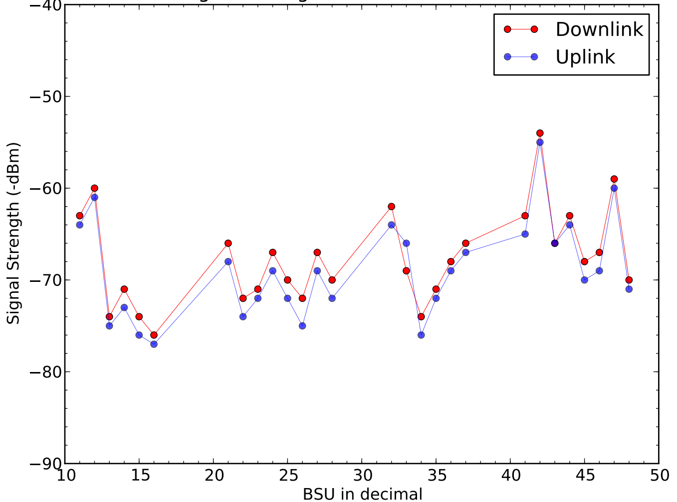
Signal Strength of BSU on 2016-04-15
