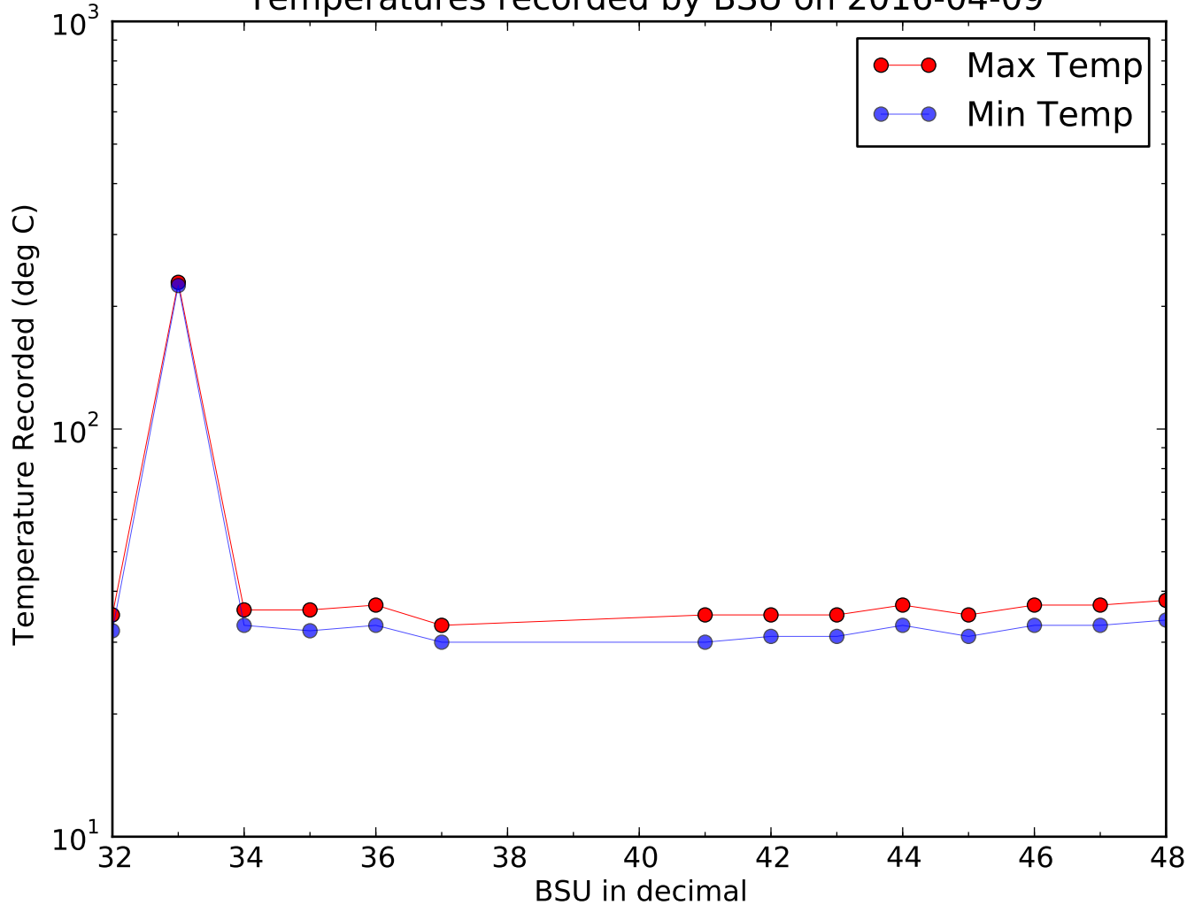
Temperatures recorded by BSU on 2016-04-09
