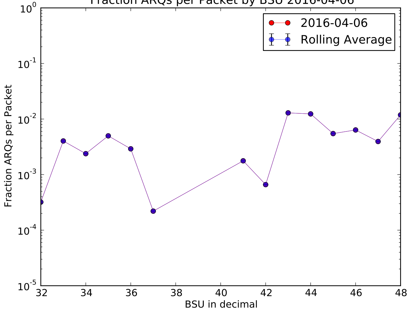
Fraction ARQs per Packet by BSU 2016-04-06
