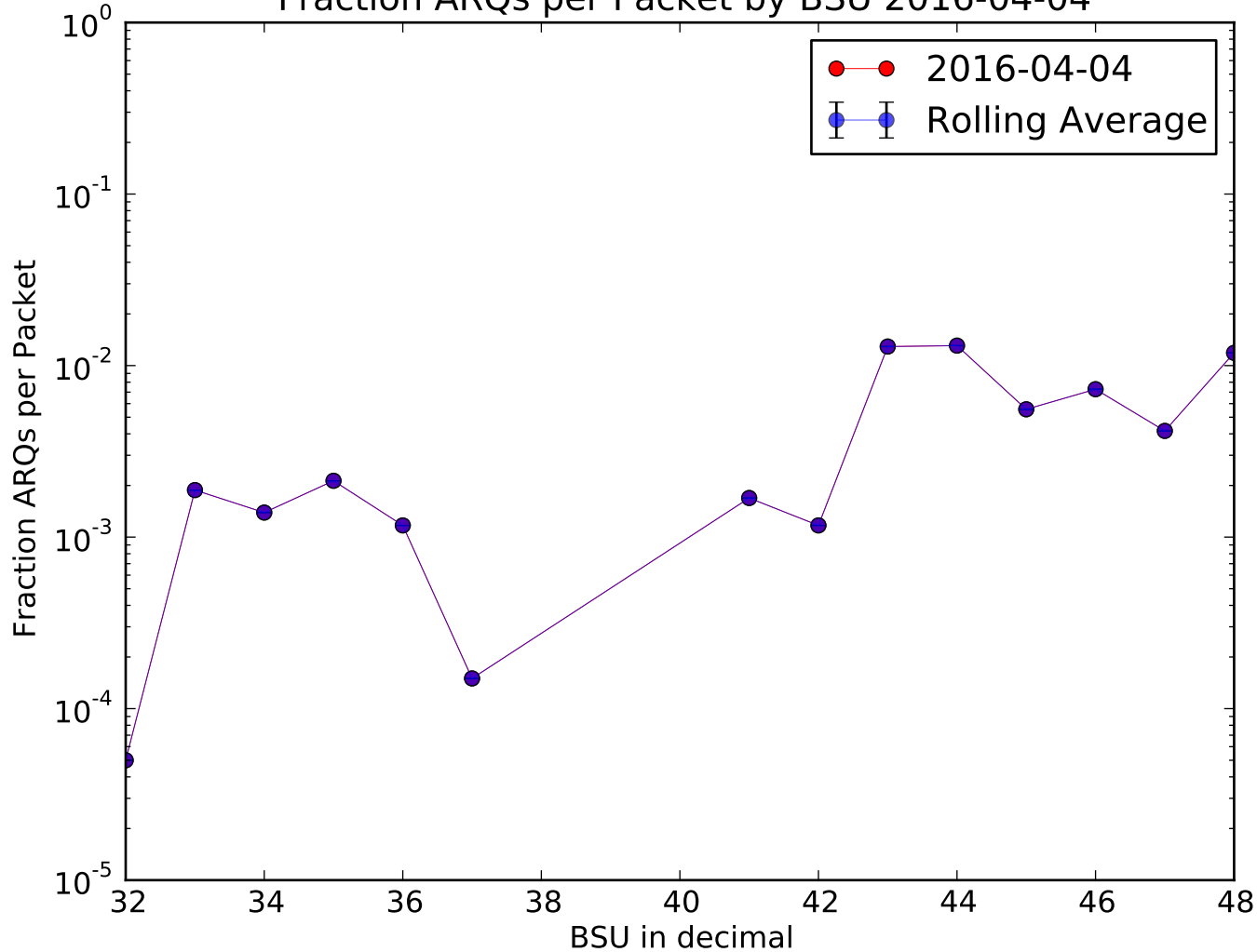
Fraction ARQs per Packet by BSU 2016-04-04
