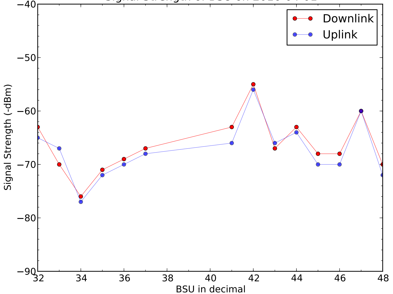
Signal Strength of BSU on 2016-04-01
