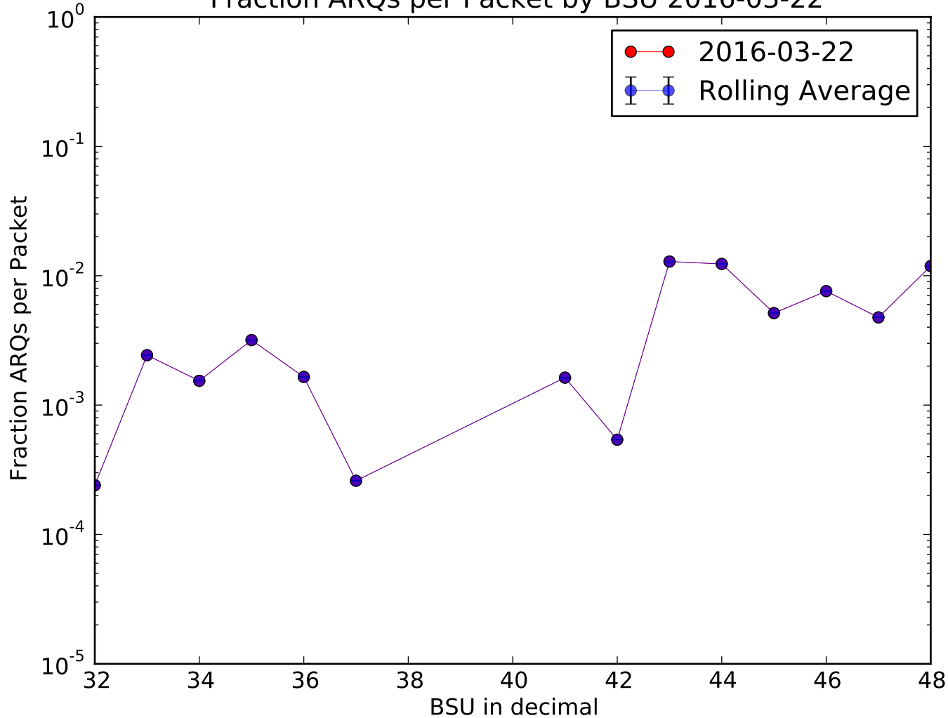
Fraction ARQs per Packet by BSU 2016-03-22
