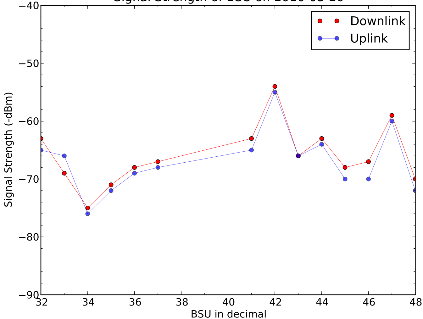
Signal Strength of BSU on 2016-03-20
