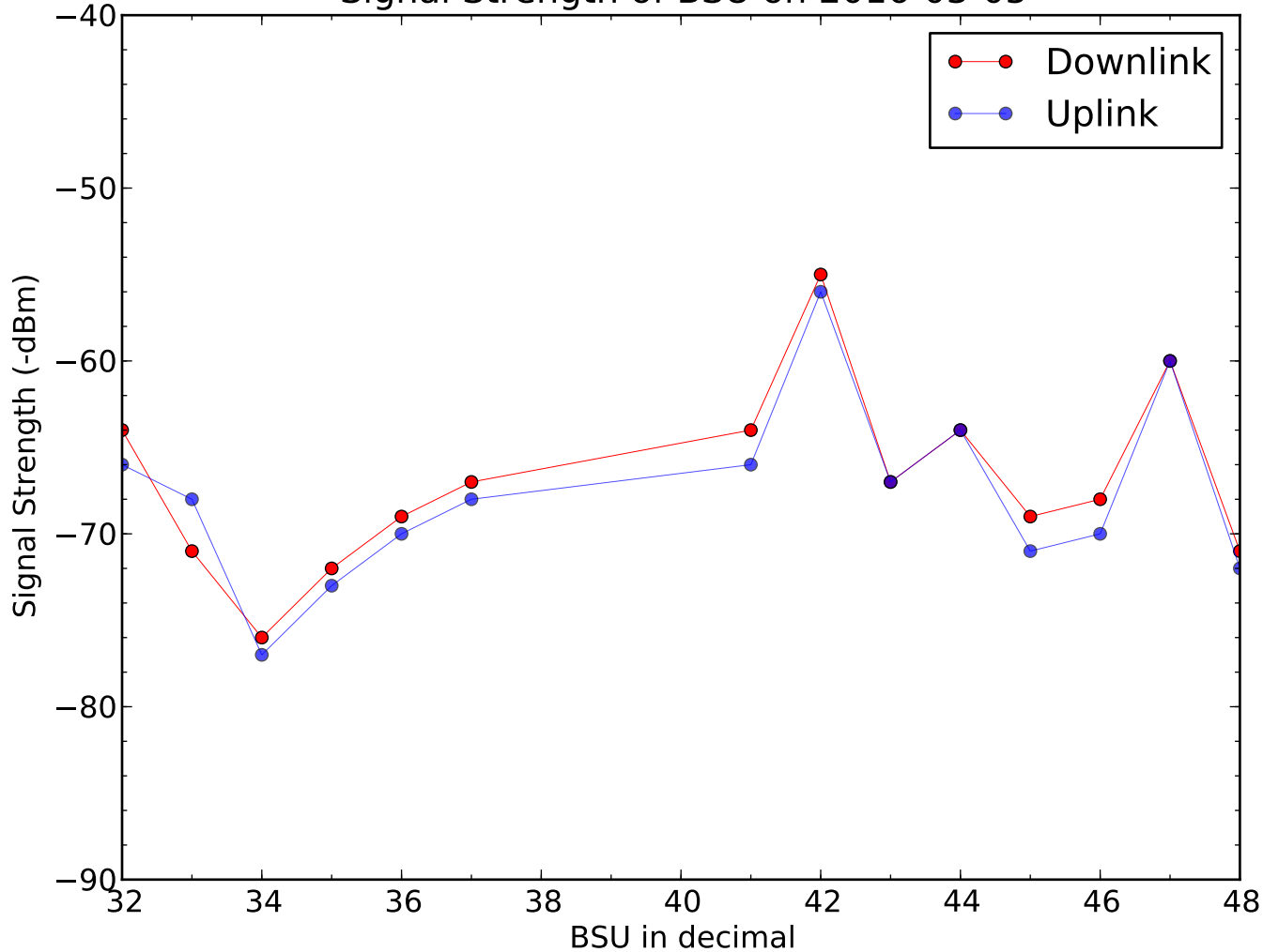
Signal Strength of BSU on 2016-03-05
