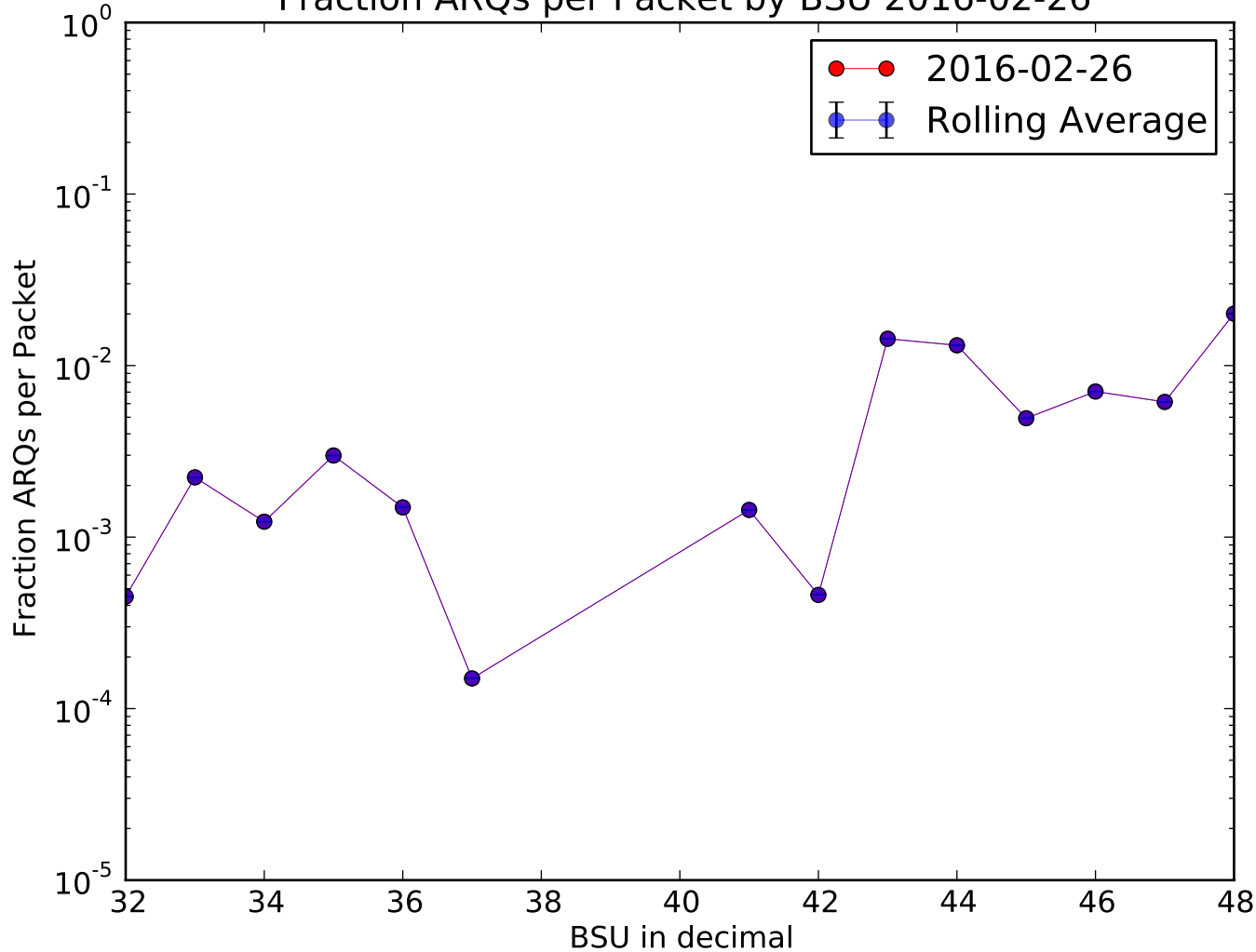
Fraction ARQs per Packet by BSU 2016-02-26
